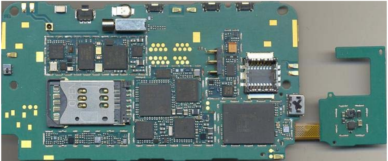
Integrated WLAN module
